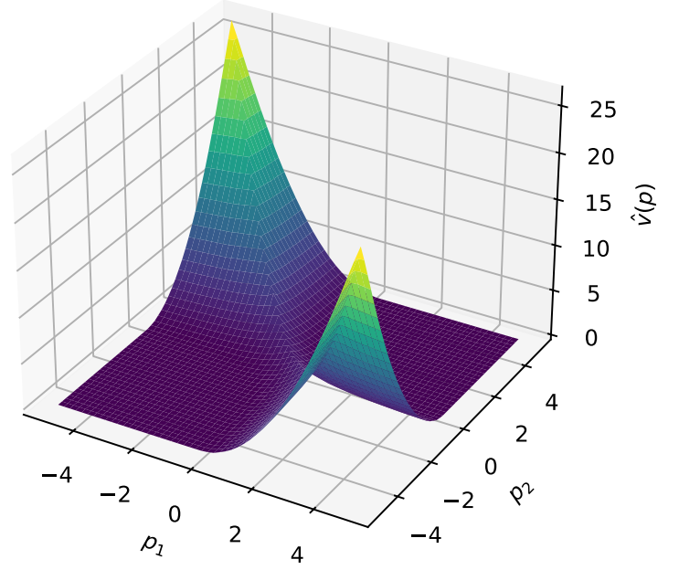
Figure 3. Neural network-based value function predictions over target parameter subspace \Phi = [-5, 5] \times [-5, 5] for problem (14).
