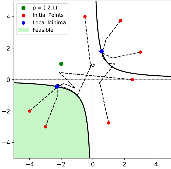
Figure 2. IPM convergence behavior for problem (14) for p = (-2, 1) . The global minimum is near (-2.3, -0.5) , while a spurious local minimum is near (0.6, 1.8) .
