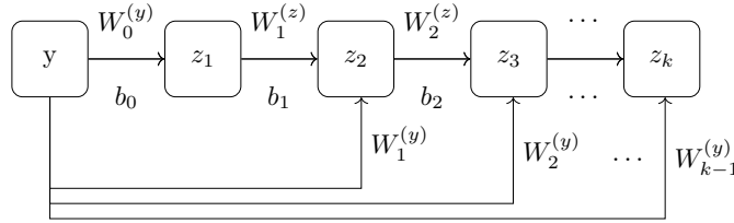
Figure 4. Neural network with skip connections.
